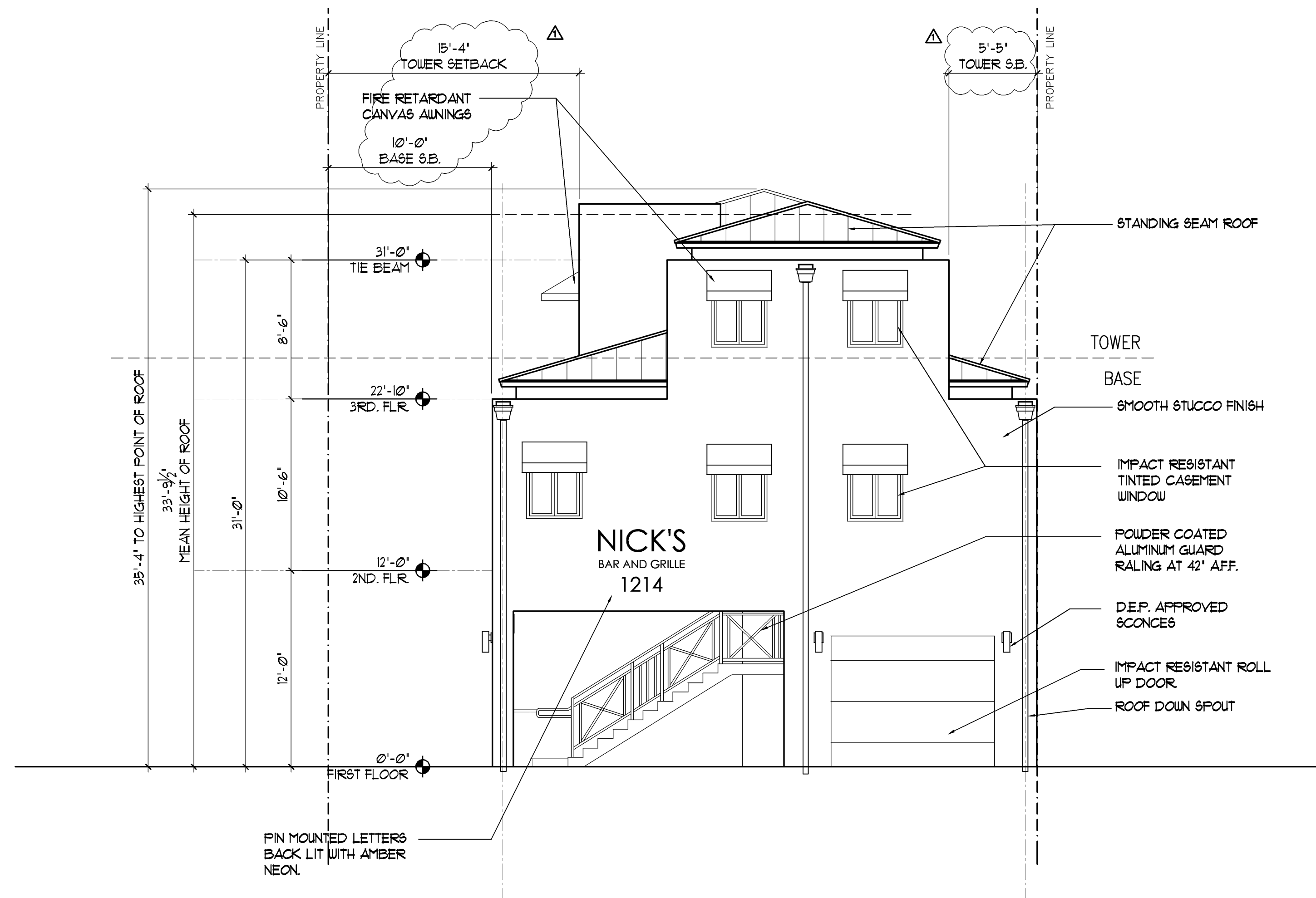
1 | PROPOSED WEST ELEVATION
