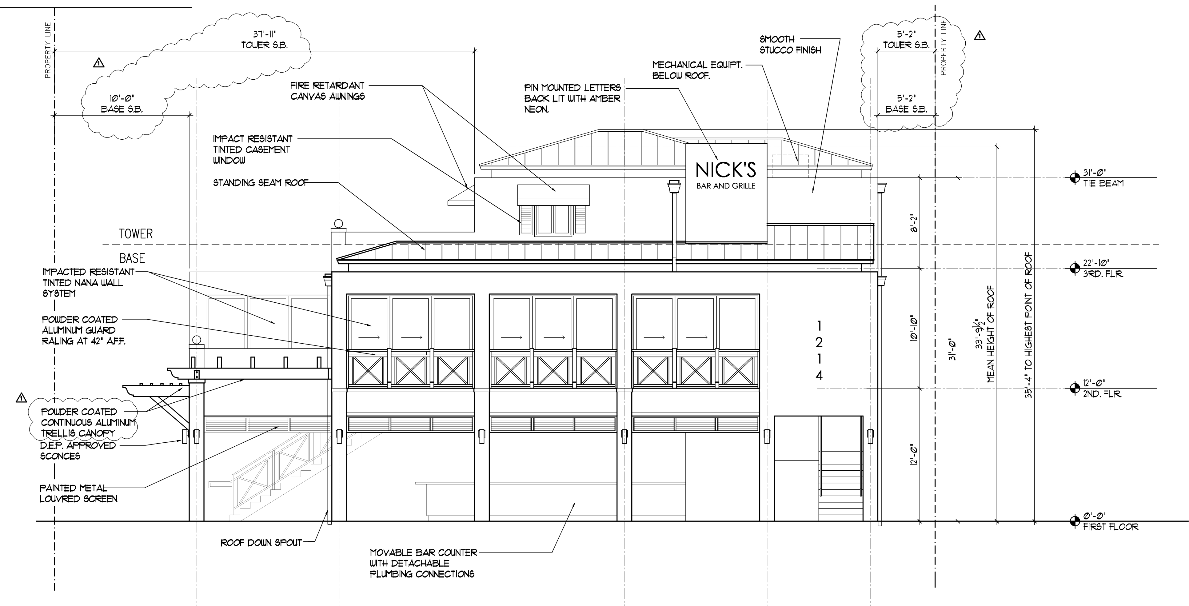
2 | PROPOSED NORTH ELEVATION
