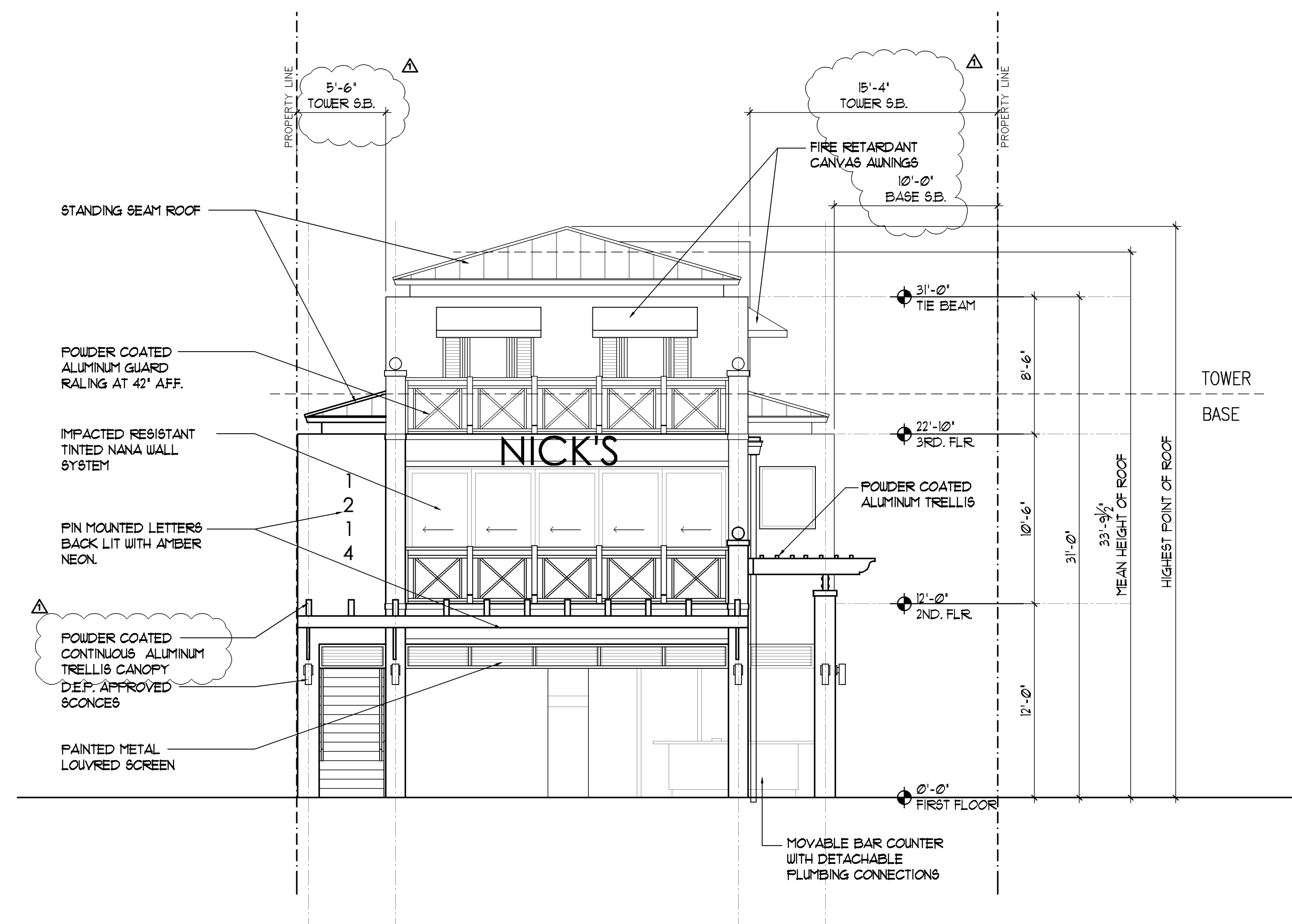
1 | PROPOSED EAST ELEVATION
